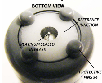
S651CD-ORP
