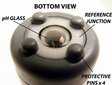
S651CD(pH)
